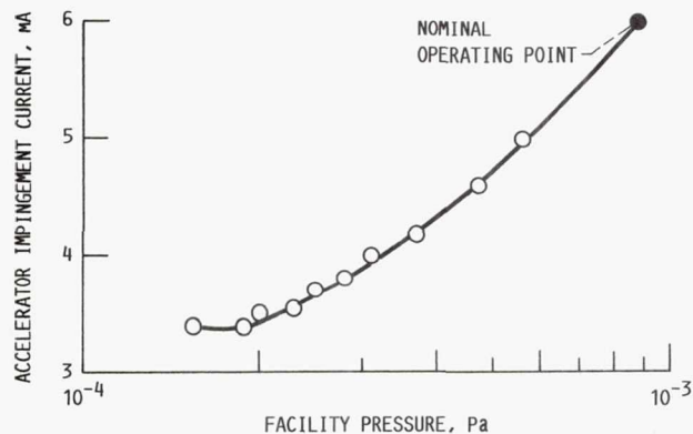
FIGURE 7. - ACCELERATOR IMPINGEMENT CURRENT AS A FUNCTION OF FACILITY PRESSURE (CONSTANT BEAM CURRENT OF 0.7 A, TWO-GRID 25 CM THRUSTER).
