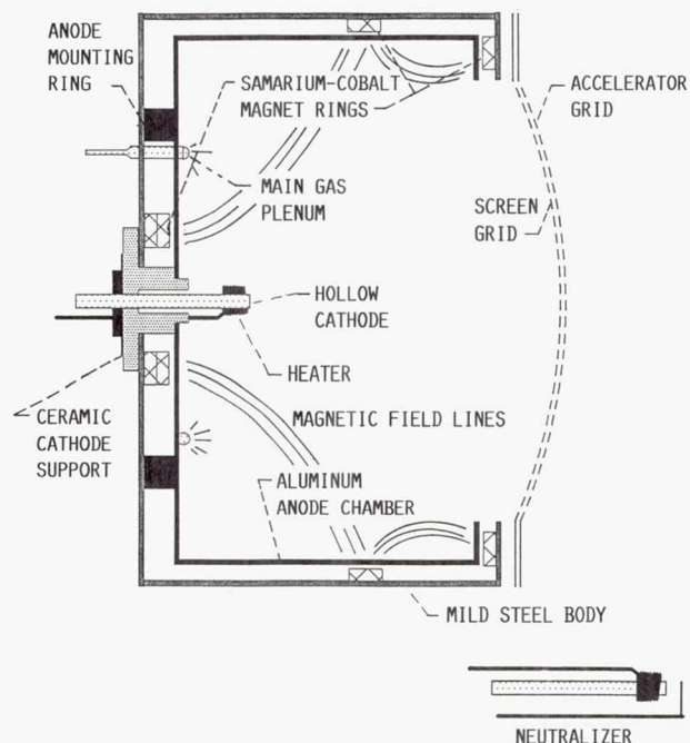
FIGURE 2. - TYPICAL RING-CUSP ION THRUSTER.
