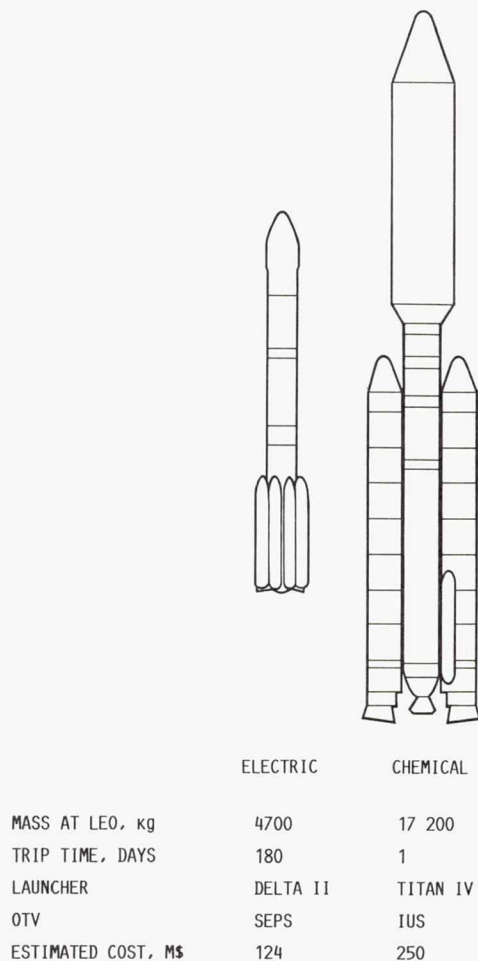
FIGURE 1. - IMPACTS OF ADVANCED ORBIT TRANSFER PROPULSION (REF. 3).
