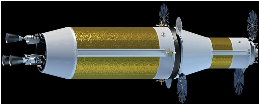
Figure 11. Key LANTR LTV System Elements – the \text{LH}_2 NTPS and In-Line \text{LO}_2 Tank
