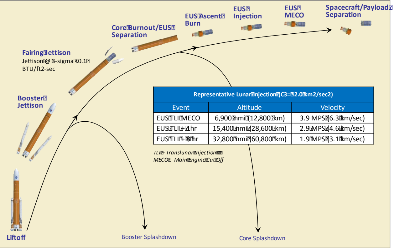
Figure 4-3. Nominal SLS Block 1B Ascent Profile
