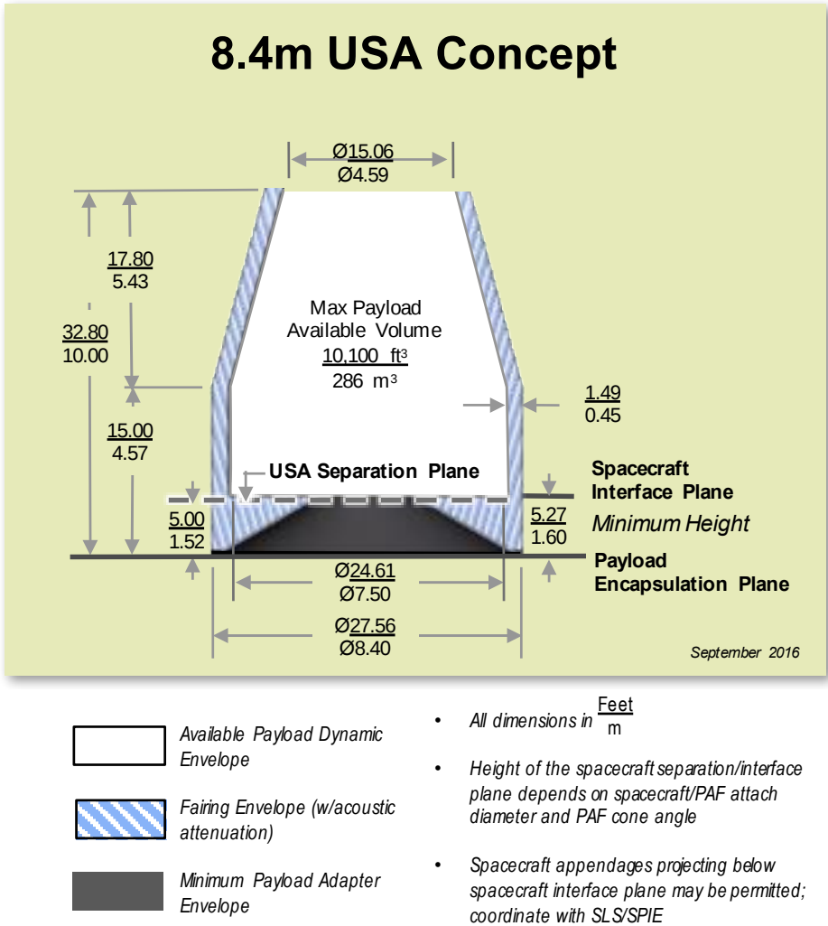
Figure 6-4. Composite Universal Stage Adapter Concept
