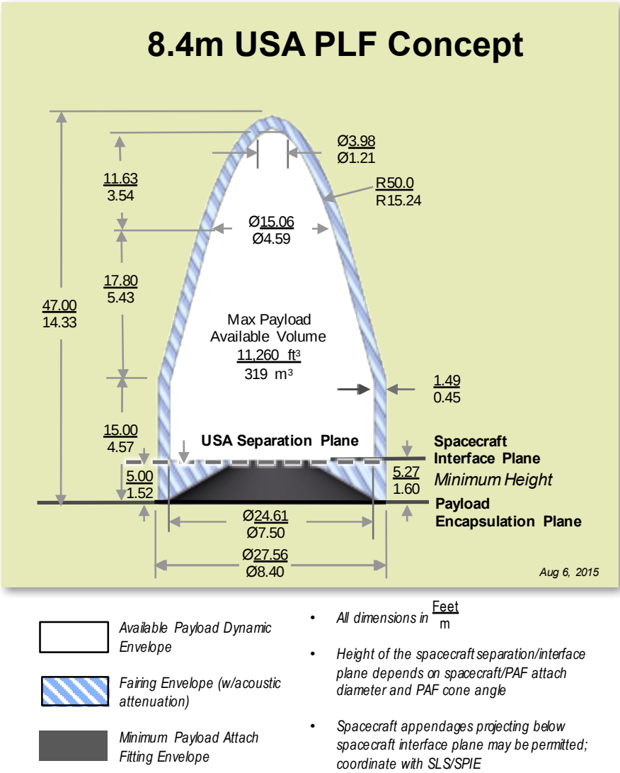
Figure 6-6. Composite 8.4m USA PLF Concept
