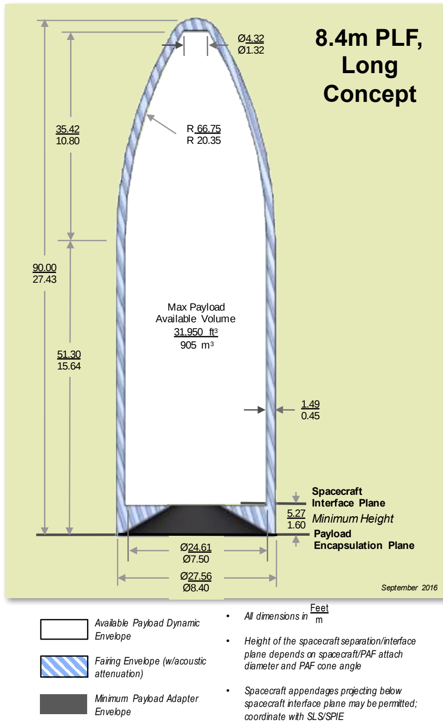
Figure 6-9. Composite 8.4 m PLF, Long Concept
