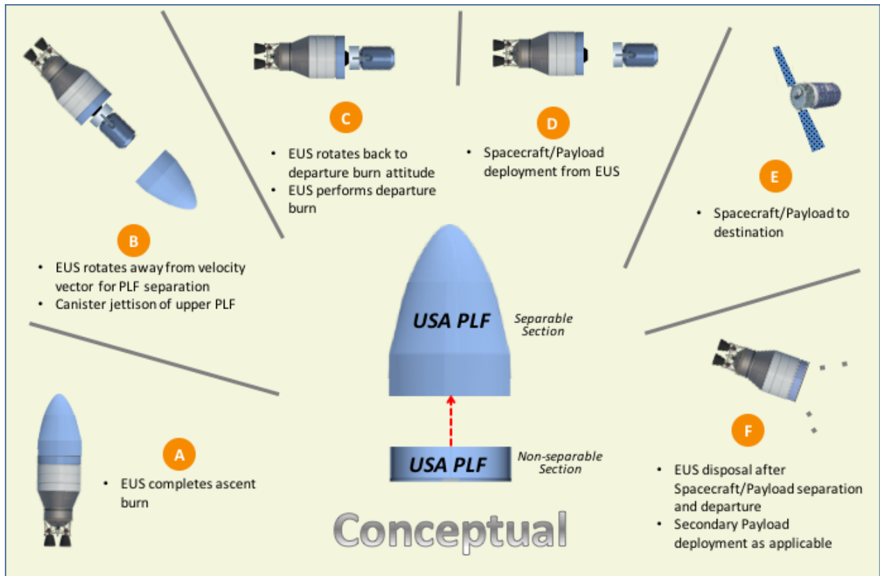
Figure 6-7. Composite 8.4m USA PLF Concept of Operations
