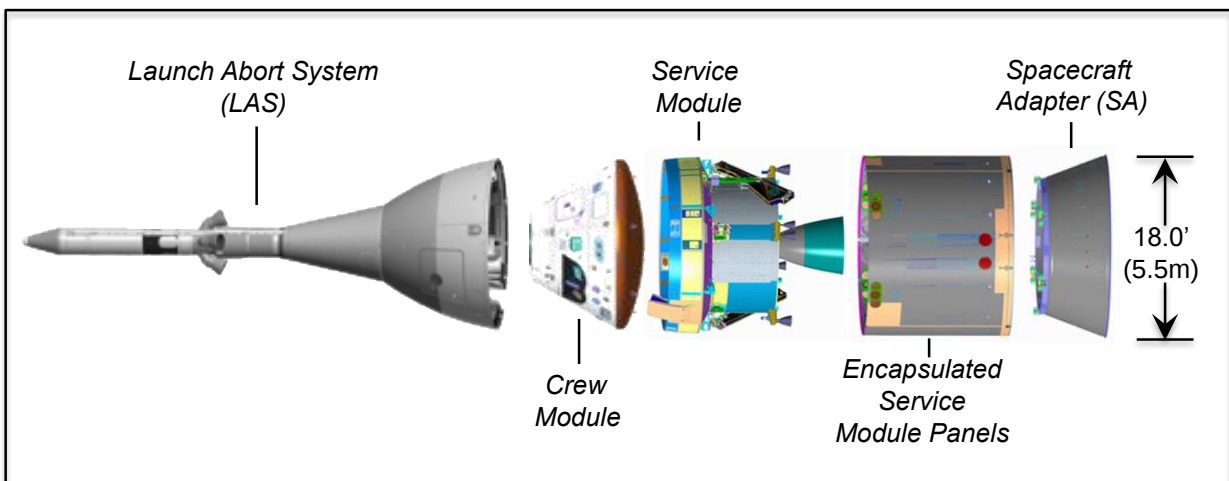
Figure 6-3. SLS to Orion Interfaces for Crewed Missions
