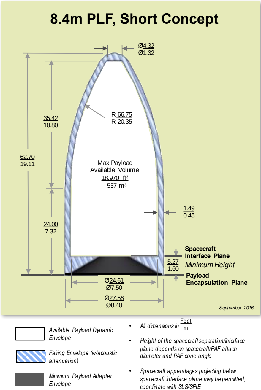
Figure 6-8. Composite 8.4 m PLF, Short Concept
