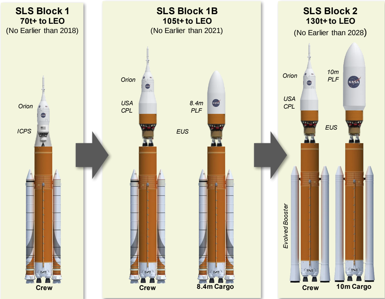
Figure 3-2. SLS Block Configurations
