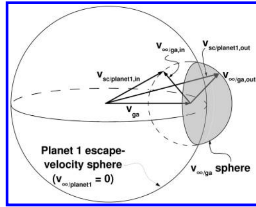
Fig. 2 Flyby vector diagram of a gravity assist from a satellite.
