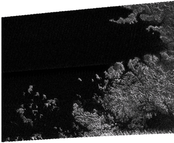
Figure 2.2-2. A wealth of organic molecules are expected to be dissolved in the hydrocarbon seas of Titan. In this 160 km by 270 km view a northern sea floods coast lines with what is presumed to be mostly liquid methane and ethane.
