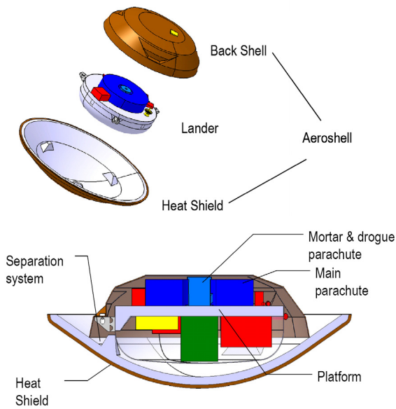
Figure 3.2-6. Conceptual design of the lake lander in the stowed configuration. An exploded view of the Huygens heritage entry aeroshell is shown.
