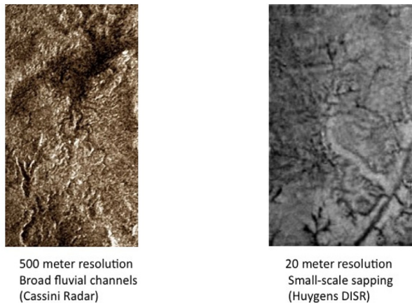
Figure 2.4-1. Cassini coverage at large scales at 350–500 m resolutions shows areas of fluvial erosion but not the details of its style (left). The Huygens probe has revealed, at 10–20 m resolution, both dendritic-type fluvial erosion and what appears to be sapping of “ground-methane” (right).
