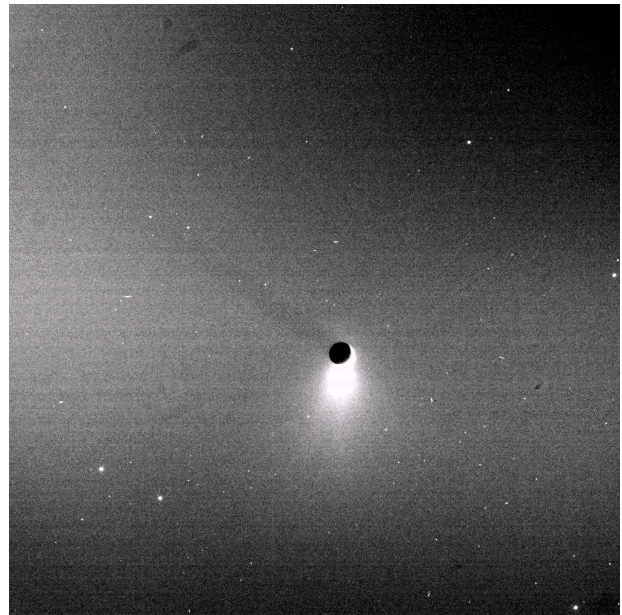
Figure 2.2-3. Looking like a comet, Enceladus shows its plume in scattered sunlight as this moon casts a shadow some 500 km across on the rings of Saturn. Cassini ISS image. NASA/JPL/Space Science Institute.
