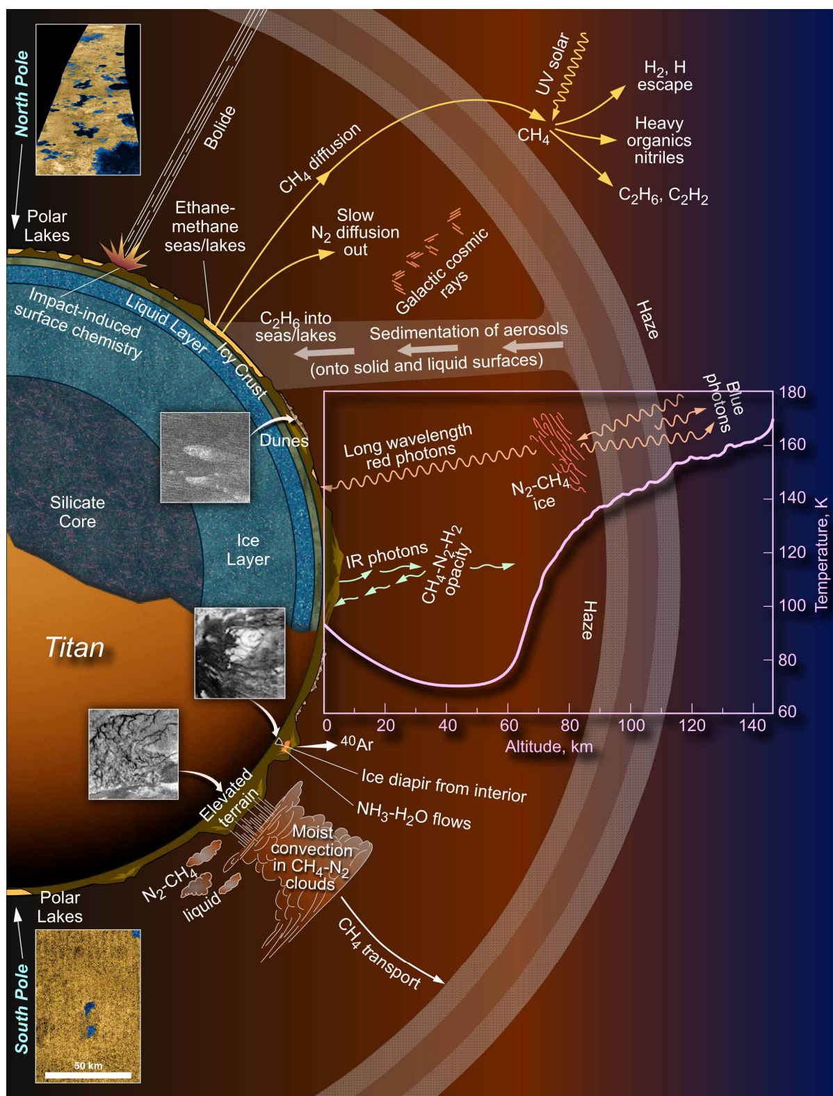
Figure 2.2-1. Schematic illustration of the connections among Titan's interior, surface, atmosphere, and cosmic environment. Processes illustrated are confirmed or strongly implicated to be occurring on the surface. Images show lakes at north and south.
