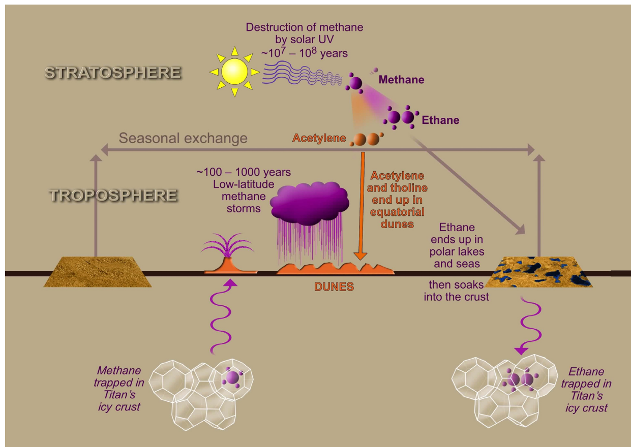
Figure 2.1-1. A schematic view of the methane cycle on Titan shown with rough timescales for the various processes.
