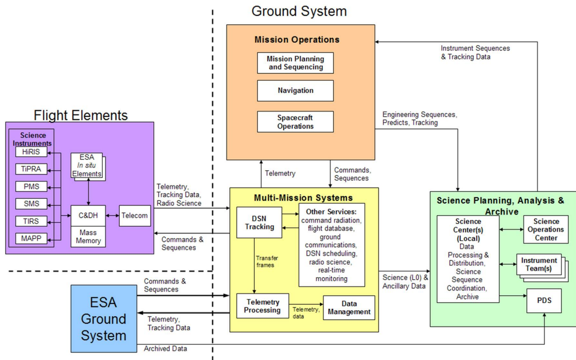
Figure 3.2-8. Proven NASA and ESA Ground Systems ensure maximum science data return.
