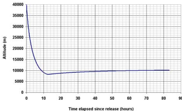
Figure 3.2-4. System modeling of the montgolfière descent profile indicates establishment of safe and stable float altitude of 10 km following balloon deployment at 40 km.
