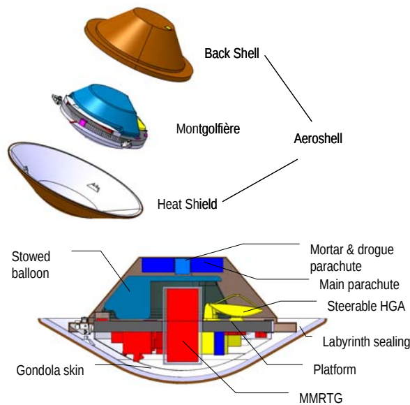
Figure 3.2-3. Conceptual design of the montgolfière integrates Huygens heritage with balloon element. An exploded view of entry system aeroshell is shown.
