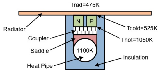
Figure 3.—Thermoelectric converter concept.
