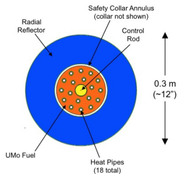
Figure 2.—Reactor radial cross section.
