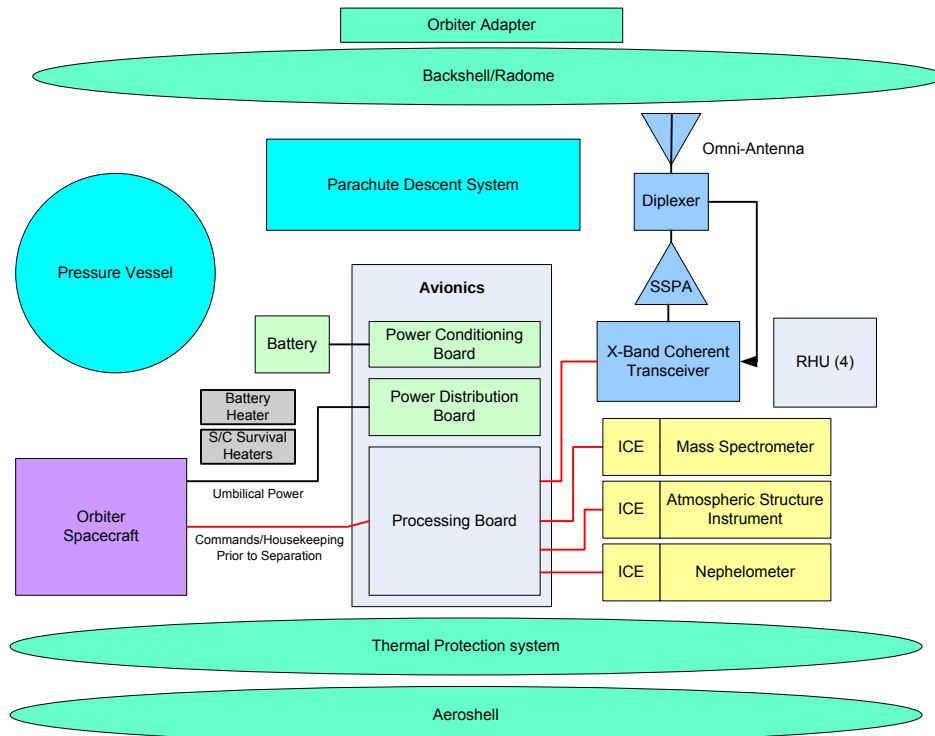
Figure 3-6. Entry probe block diagram.
