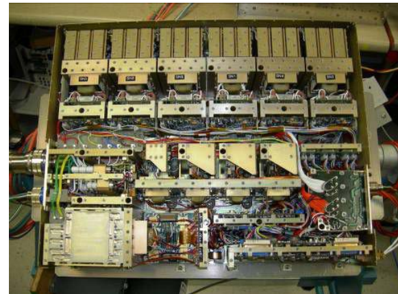
NEXT Modular Power Processing Unit
