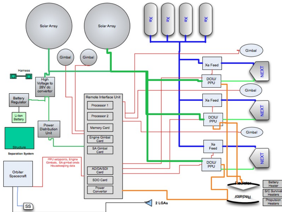
Figure 3-2. SEP stage block diagram.
