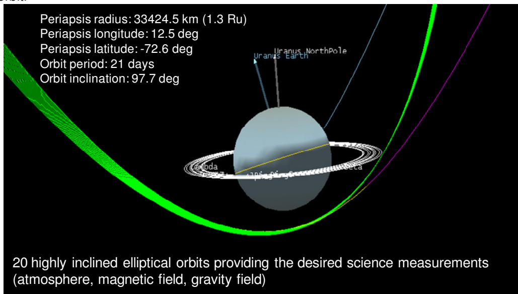
Figure 3-10. Primary science orbit.
