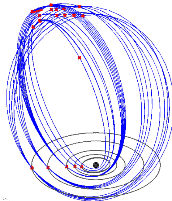
Figure 3-12. Satellite tour geometry.
