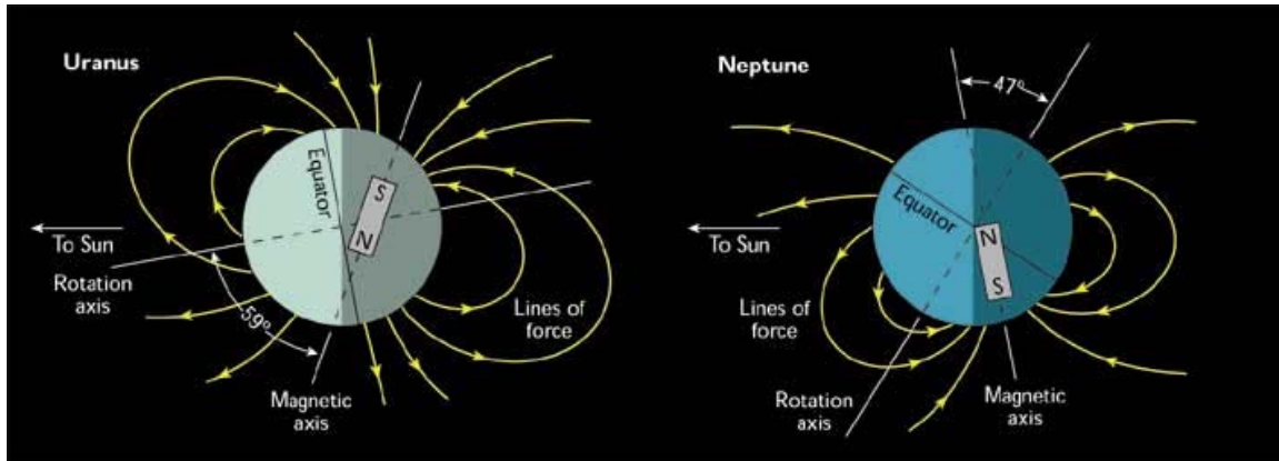
Figure 1-3. Magnetic and rotation axes of Uranus (left) and Neptune (right).
