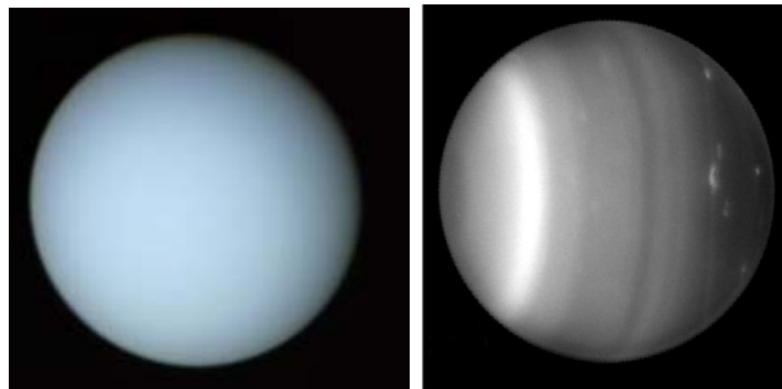
Figure 1-2. Uranus as seen by Voyager 2 in 1986 (left) and Keck in 2003 (right).
