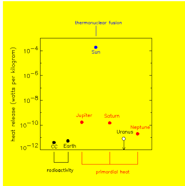
Figure 1-1. Internal heat emission of the ice giants.
