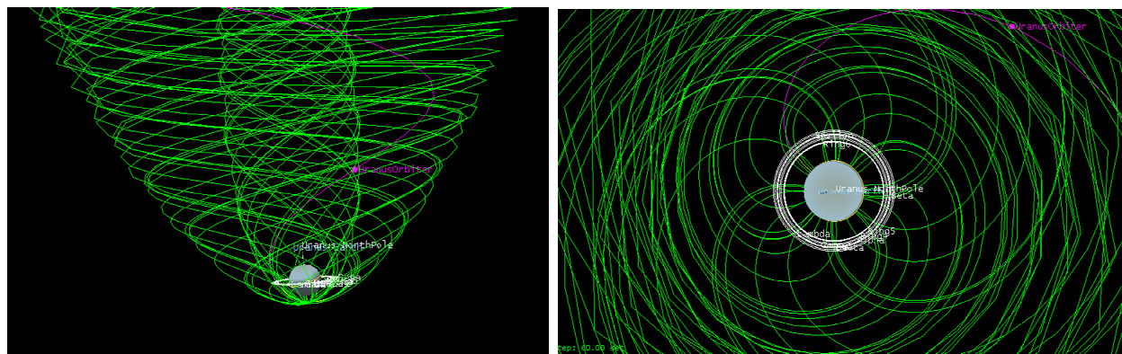
Figure 3-11. 20 Science orbits plotted in Uranus fixed coordinate system (purple line: incoming trajectory, green line: science orbits).
