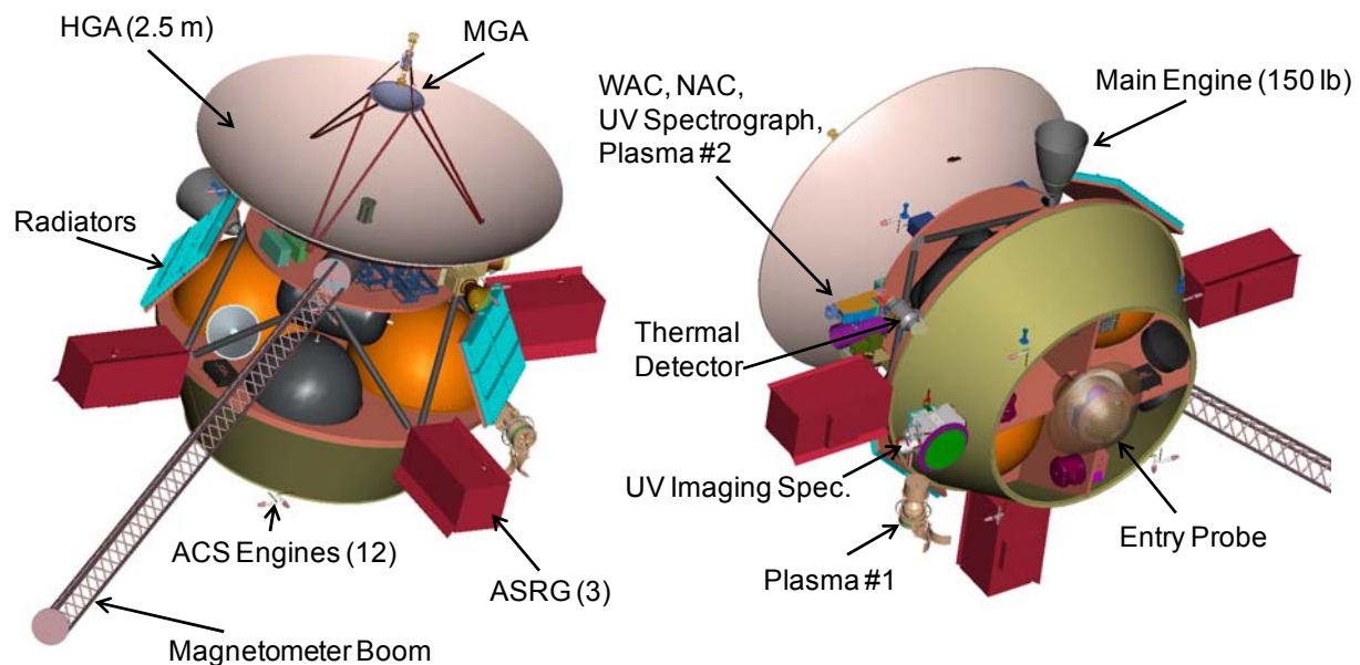
Figure 3-3. Uranus orbiter concept.
