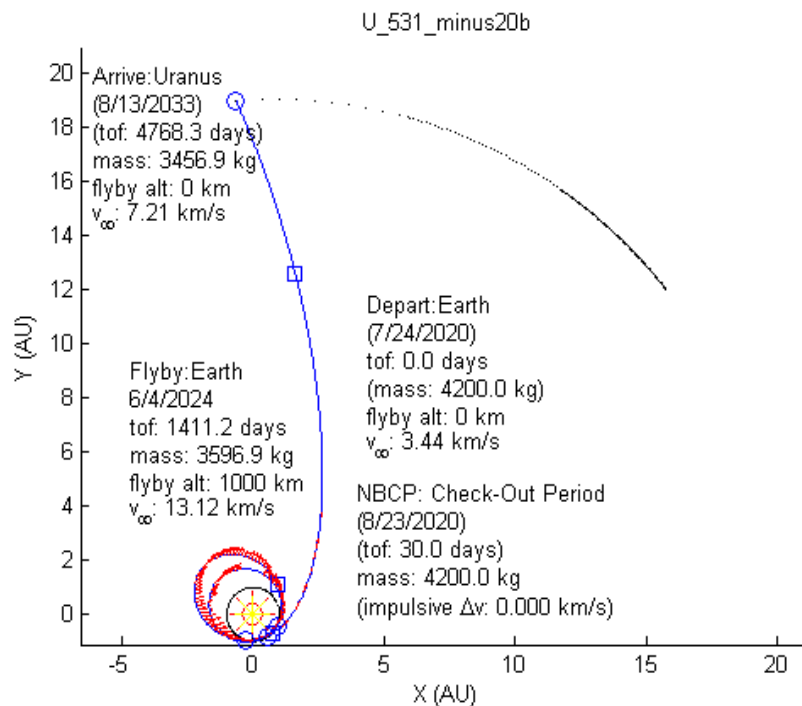
Figure 3-8. Baseline SEP trajectory for study
