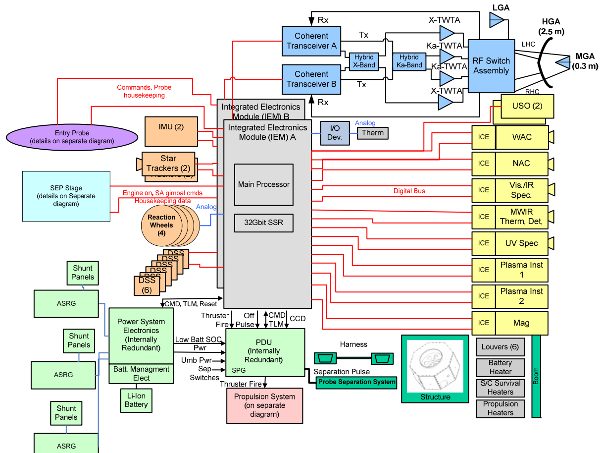
Figure 3-4. Uranus orbiter block diagram.
