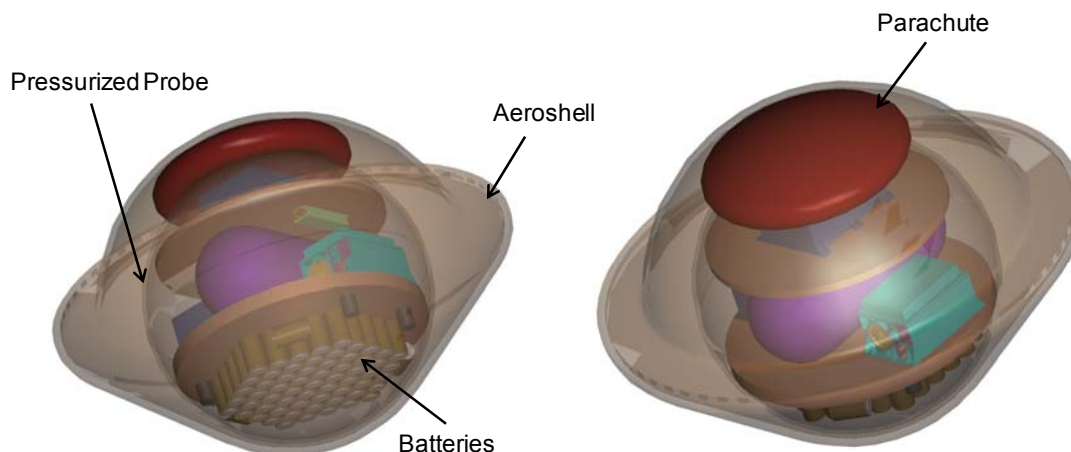
Figure 3-5. Entry probe configuration.
