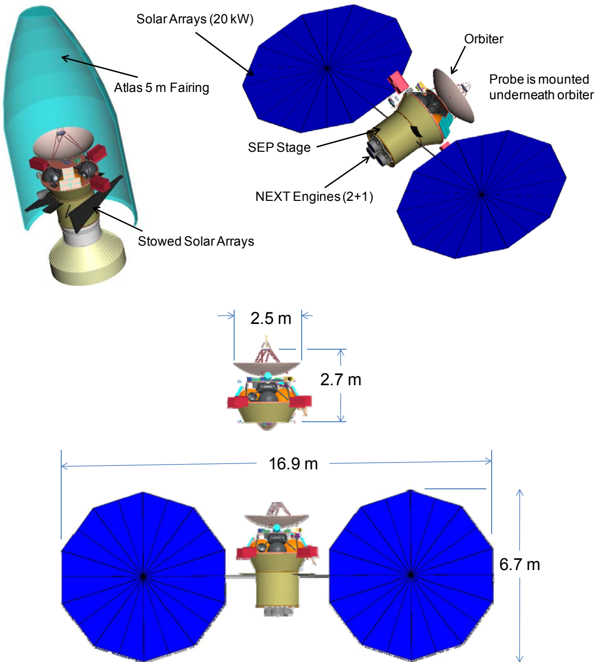
Figure 3-7. Integrated flight system: launch (upper) and SEP (lower) cruise configurations.
