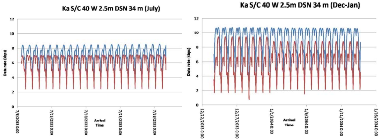
Figure 3-13. Data rate variations for two seasons with DSN.
