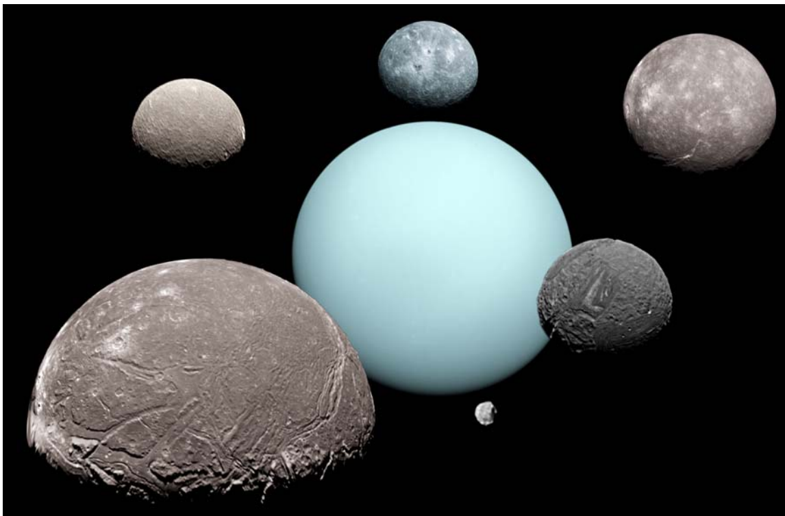
Figure 1-4. Uranus and some of its moons.
