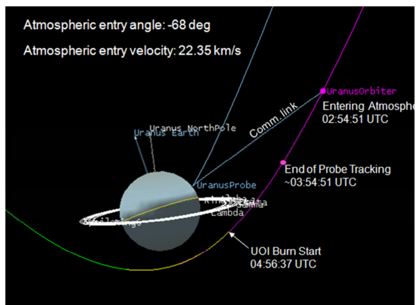
Figure 3-9. Probe entry and UOI geometry.
